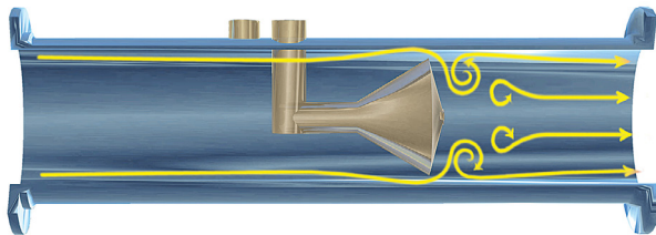
The V-Cone Built-In Flow Conditioning
