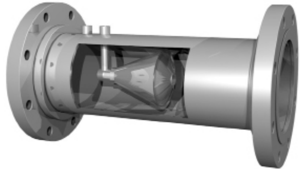
The V-Cone Flow Meter's Centrally Located Cone
