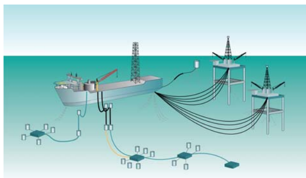
Figure 1: Subsea Overview
