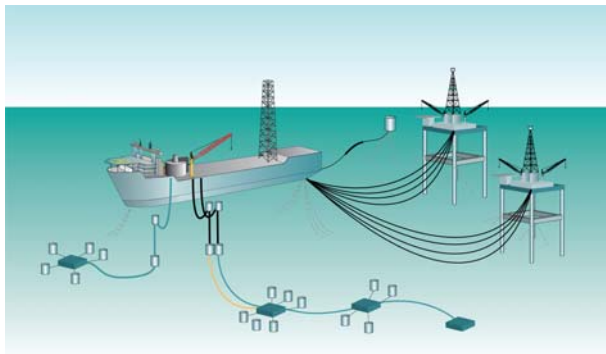
Figure 1: Subsea Overview
