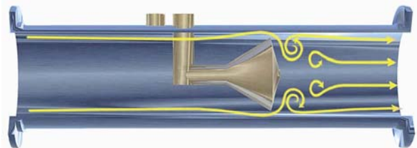
Figure 4: Vortices Created By The V-Cone
