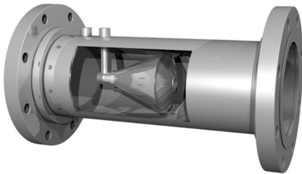
Figure 3: V-Cone Flowmeter Cutaway
