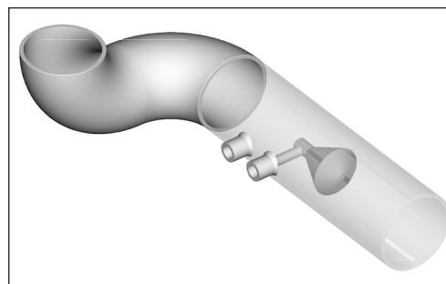
Figure 5. Coude Double et V-Cone
