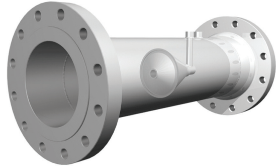
Figure 2: The V-Cone Flow Meter
