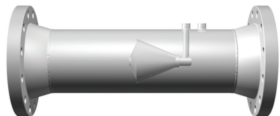
Figure 3: Cut-away side view shows the V-Cone flow meter's V-shaped conical intrusion in the center of the pipe.
